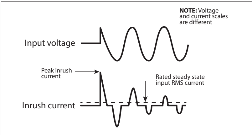
Fig 4.1: Inrush current in an SMPS
